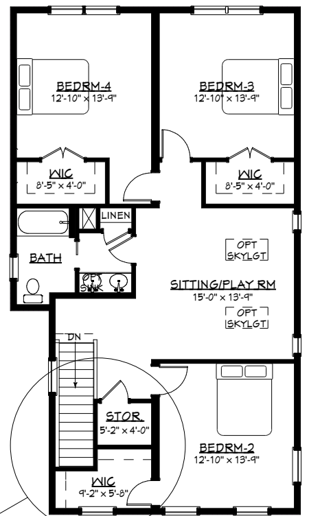
SECOND FLOOR 1,241 SF
