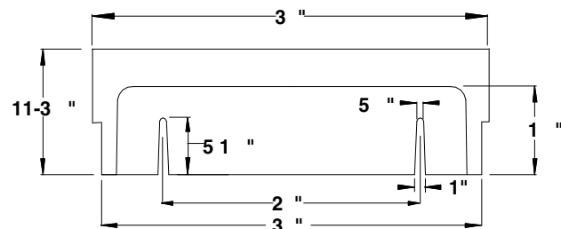
CURB HOOD FRONT VIEW
