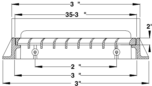
FRAME FRONT SECTION VIEW
