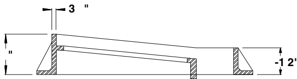
FRAME END SECTION VIEW
