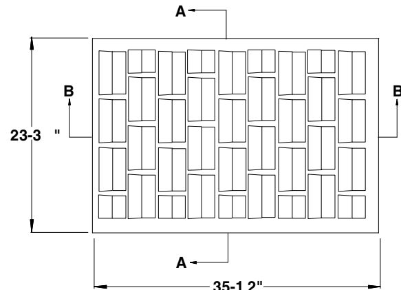
TYPE "L" GRATE TOP VIEW
