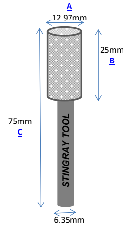
Part No.: C130-75 Vacuum Brazed
