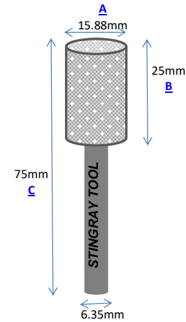
Part No.: C160-75 Vacuum Brazed
