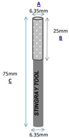
Part No.: C63-75 Vacuum Brazed
