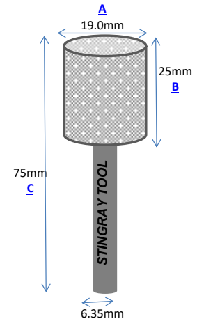
Part No.: C190-75 Vacuum Brazed
