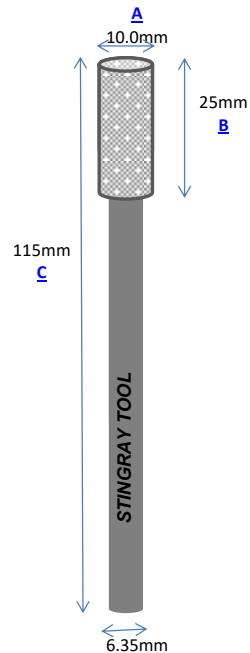
Part No.: C100-115 Vacuum Brazed
