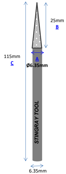
Part No.: P63-115 Vacuum Brazed
