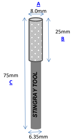
Part No.: C80-75 Vacuum Brazed
