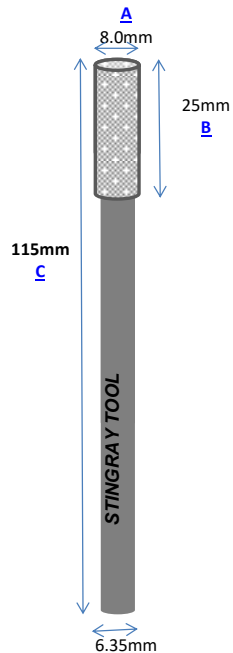
Part No.: C80-115 Vacuum Brazed
