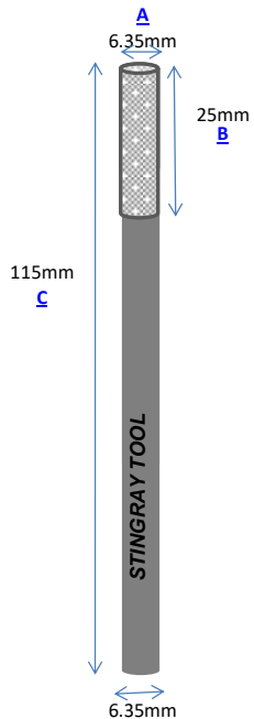
Part No.: C63-115 Vacuum Brazed
