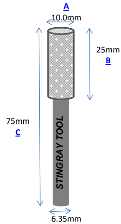
Part No.: C100-75 Vacuum Brazed
