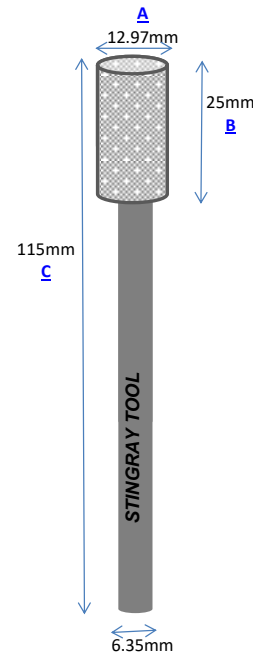
Part No.: C130-115 Vacuum Brazed
