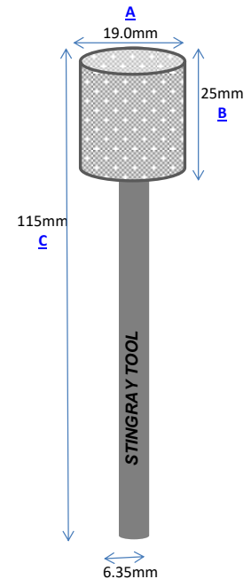
Part No.: C190-115 Vacuum Brazed
