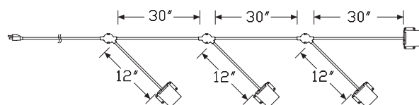
Four Power Modules
