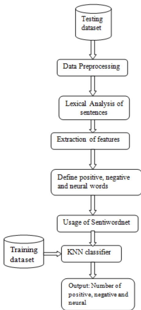
Figure 1: Proposed System Architecture
