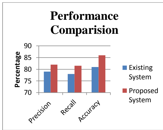
Fig 1: Performance analysis
