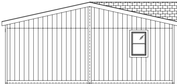
REAR ENDWALL
