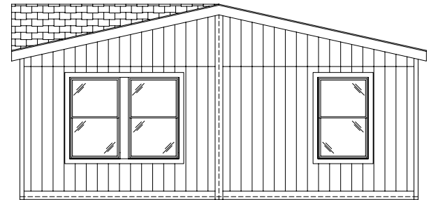
FRONT ENDWALL
