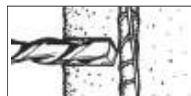
1. Stop hammer bit when rebar is encountered
