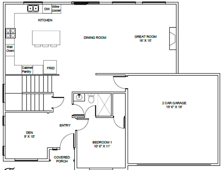
1ST FLOOR
