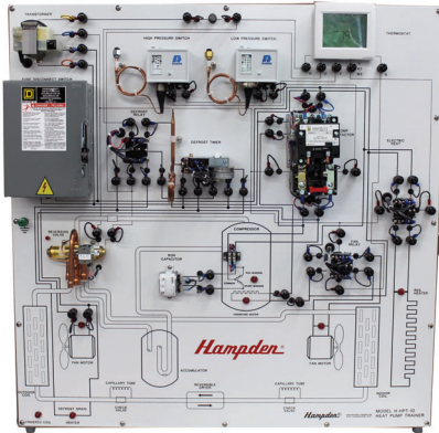
MODEL H-HPT-1D Dimensions: 36"H x 36"W x 13"D Shipping Weight: 265 lbs
