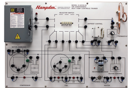
MODEL H-ACCS-2A Dimensions: 23"H x 33"W x 15"D Shipping Weight: 100 lbs
