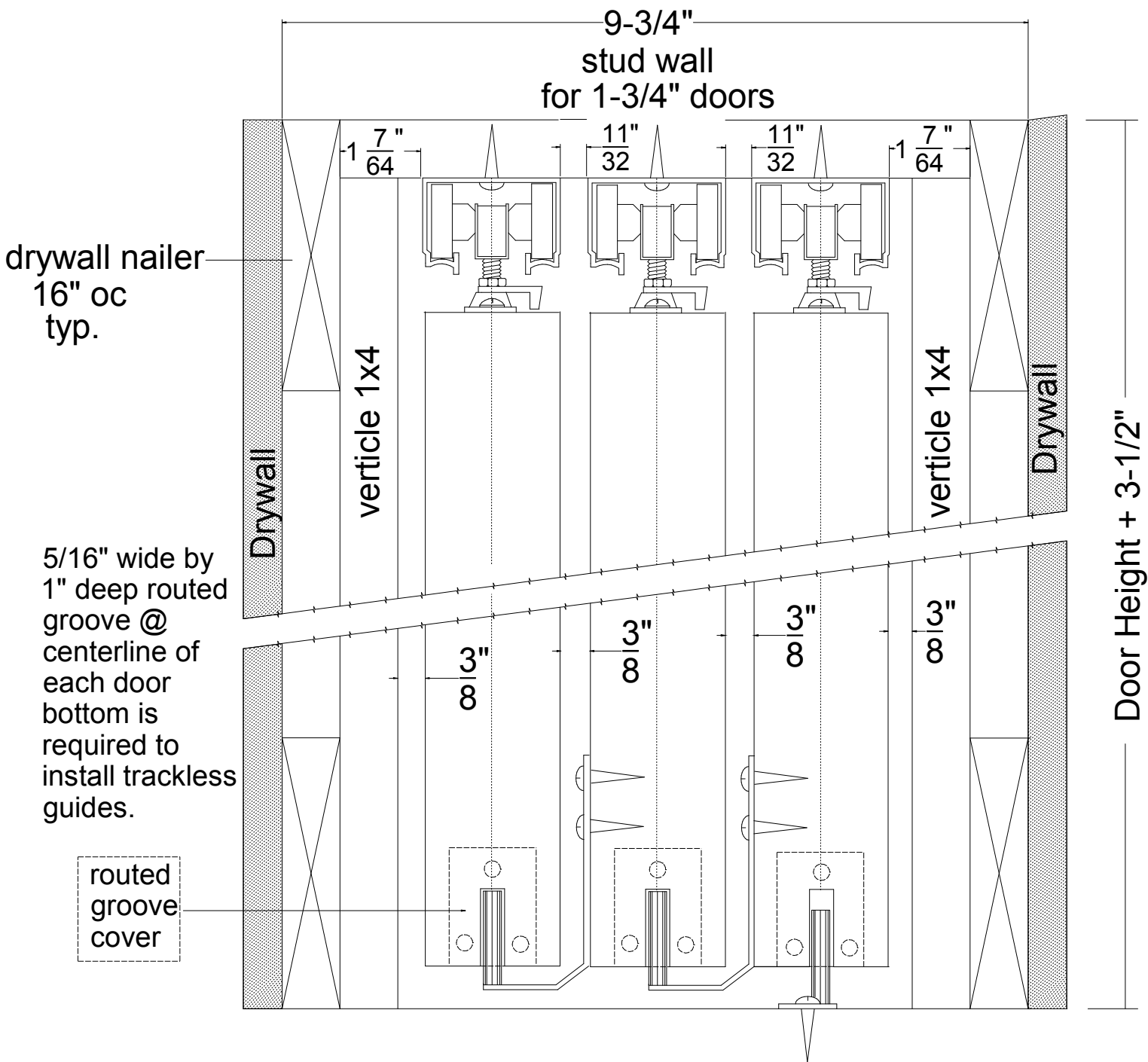
3 Door multipass frame section for 1-3/4" doors
