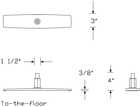
To-the-floor
