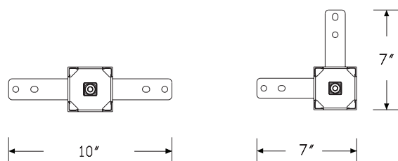
2-Way, 180 degree (2A)
