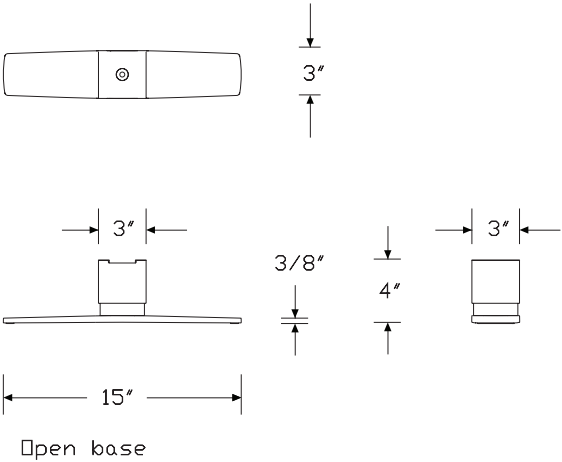
Open base
