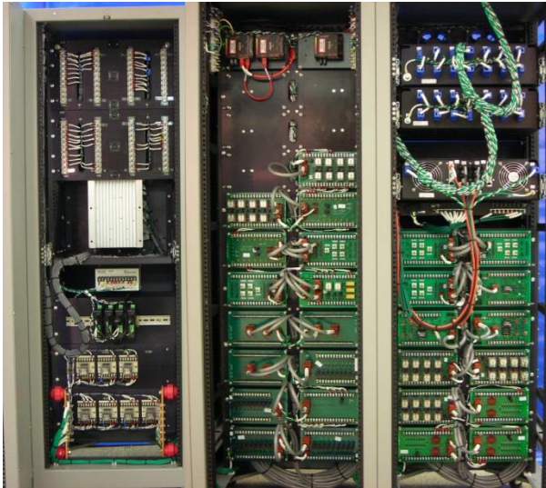
Cabinet Back
