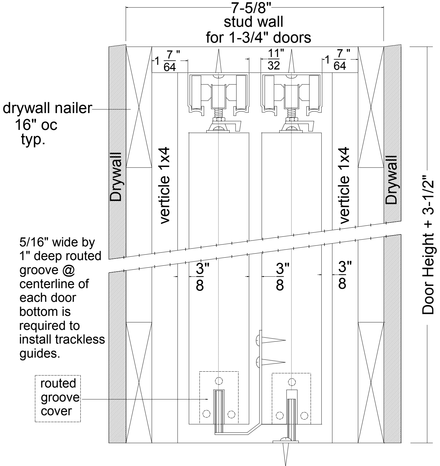
2 Door multipass frame section for 1-3/4" doors
