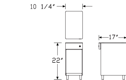
Drawer - Open with Glide
