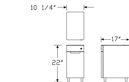
Drawer - Drawer with Glide
