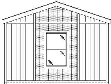
OPT. UPGRADED ENDWALL ELEVATION
