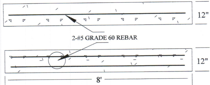
8'X12"X12" CONCRETE BASE BEAM
