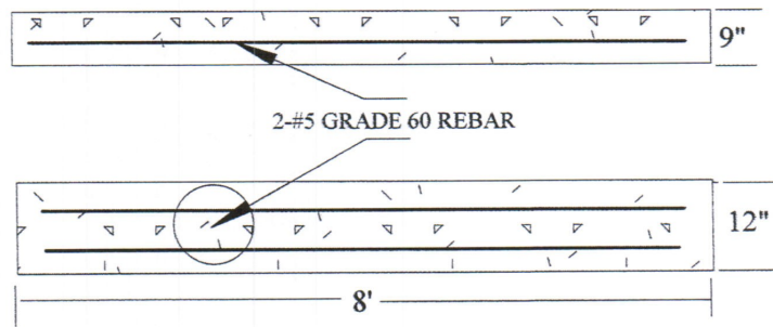
8'X12"X9" CONCRETE BASE BEAM
