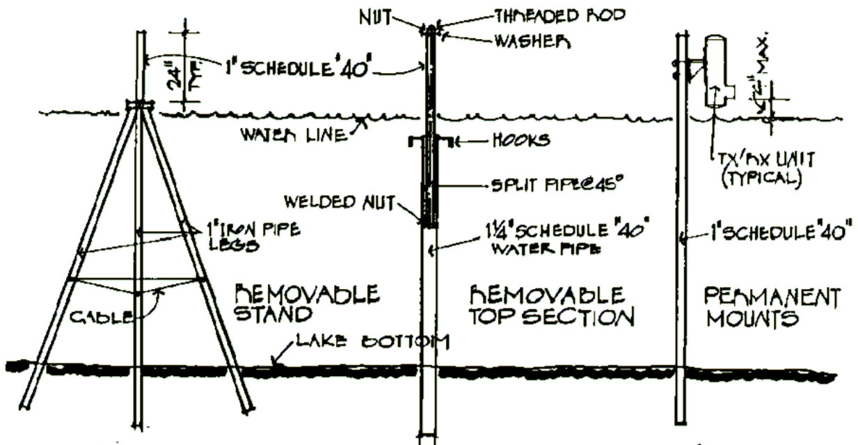
FIGURE 6 TRANSMITTER MOUNTS
