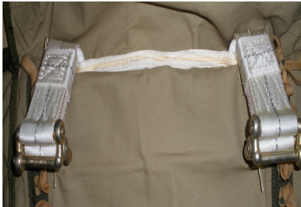
PACK TRAY INTERIOR WITH SHORT RISERS
