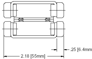
#2020 Hanger for doors up to 400 lbs
