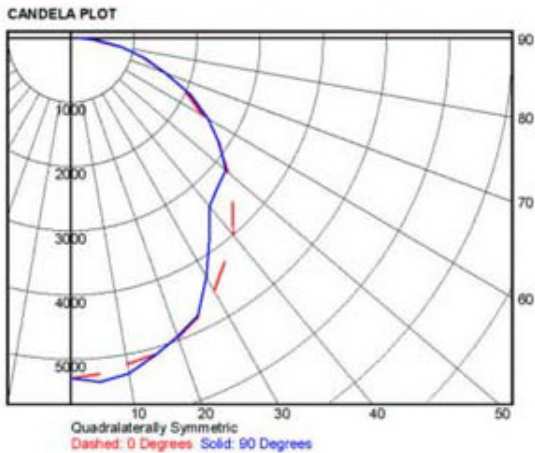
T8-8 Lamp IES File
