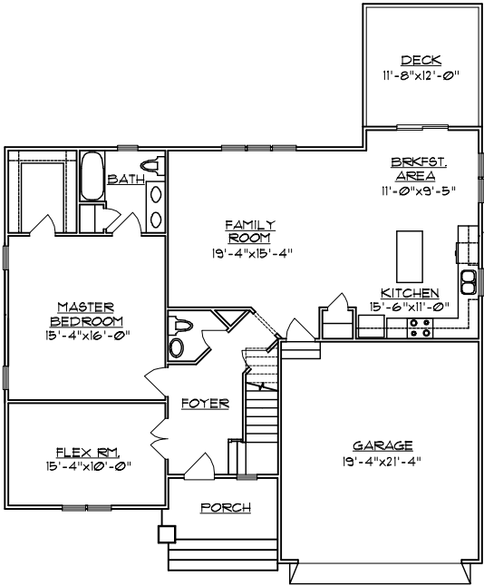
FIRST FLOOR PLAN 1318 SQ. FT. (HEATED) 429 SQ. FT. (GARAGE)
