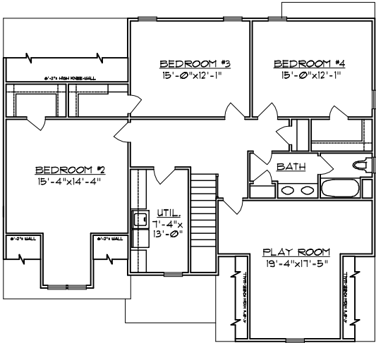
SECOND FLOOR PLAN 1164 SQ. FT. (HEATED) 267 SQ. FT. PLAYROOM (HEATED)
