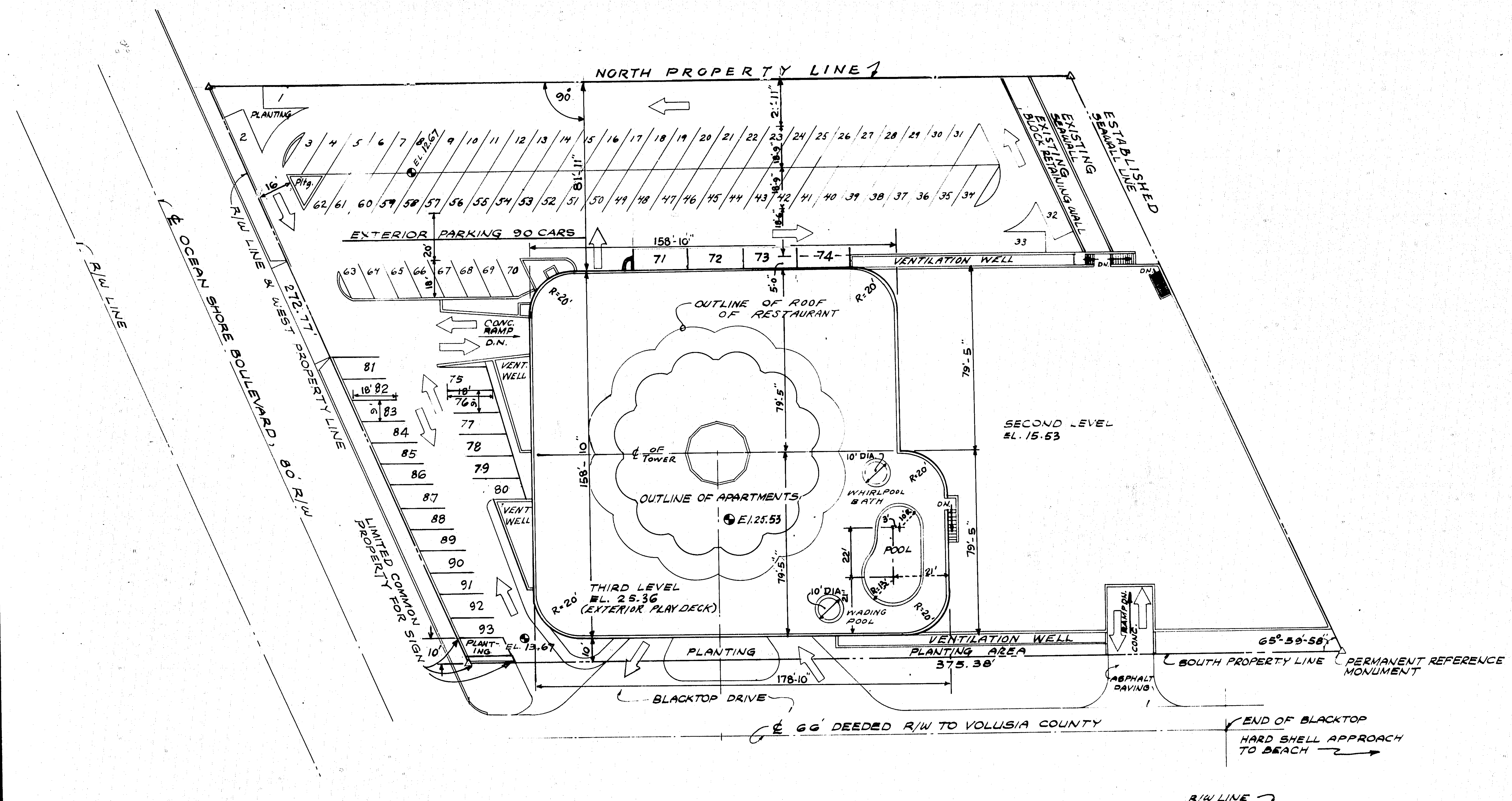
THIRD LEVEL PLAY DECK & LOT LEVEL PLAN SCALE 1 INCH = 30 FEET
