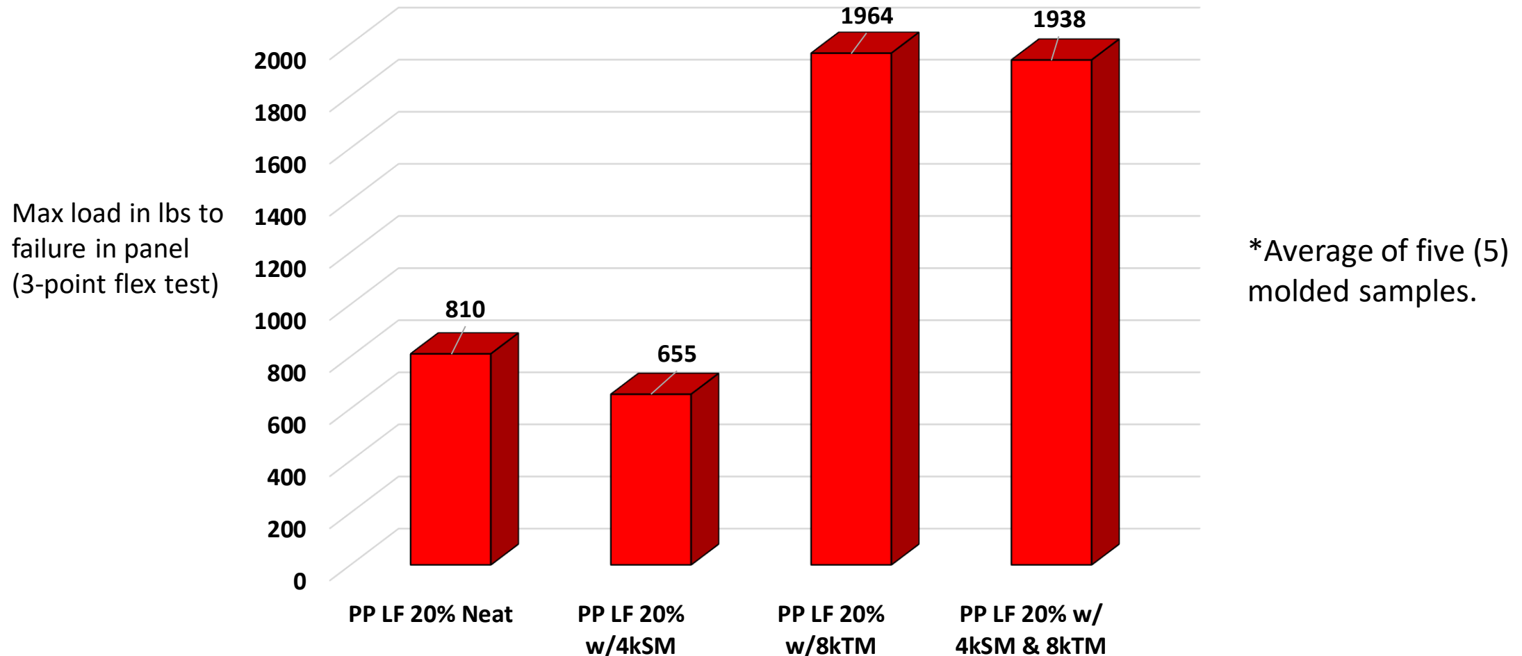
Compression Molded ICP 8"x18" Test Panels Overall Strength 3-Point Flex Testing Rib Down
