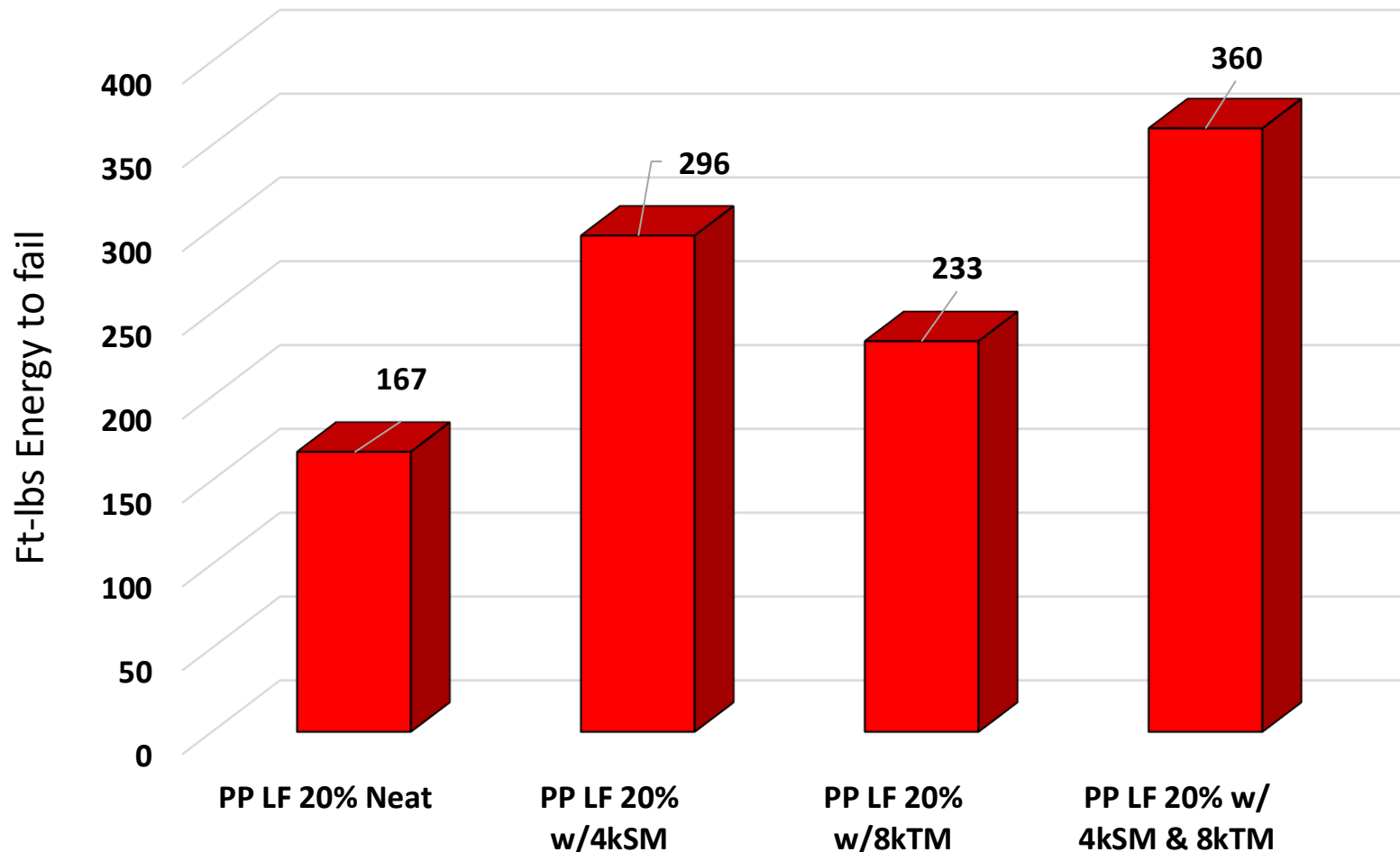
Compression Molded ICP 8"x18" Test Panels Impact Data - Pendulum Tester
