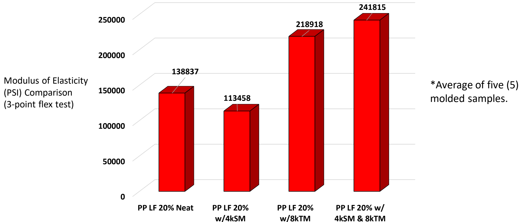
Compression Molded ICP 8"x18" Test Panels Modulus of Elasticity 3-Point Testing Rib Down
