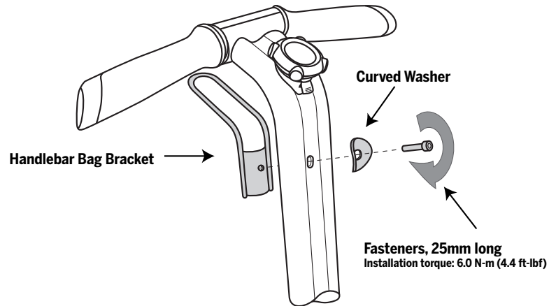
Figure 1. Installing the Handlebar Bag Bracket
