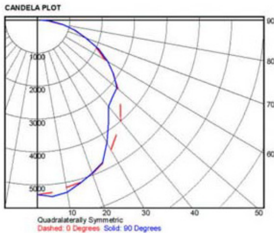
T8-6 Lamp IES File
