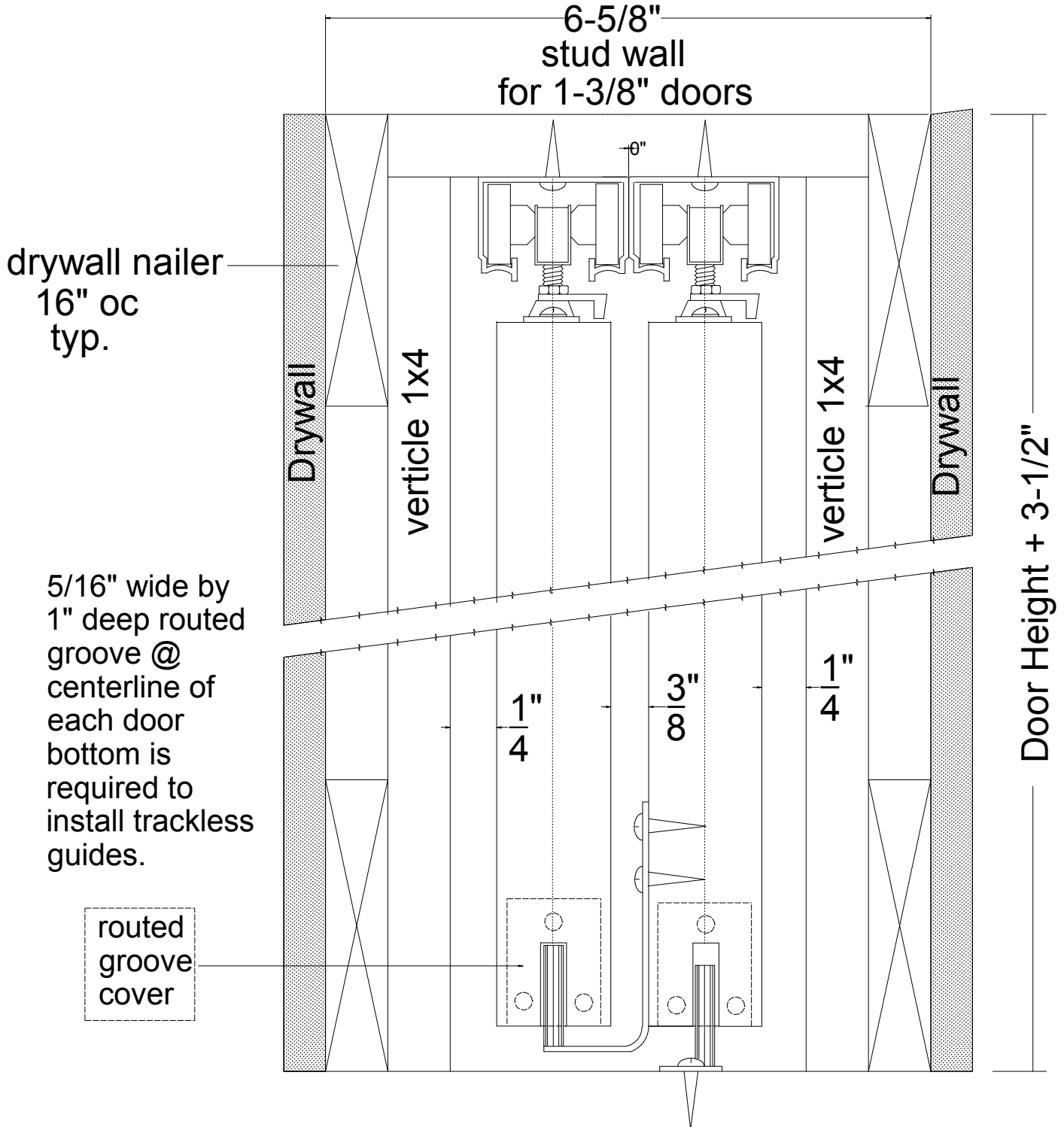
2 Door multipass frame section for 1-3/8" doors
