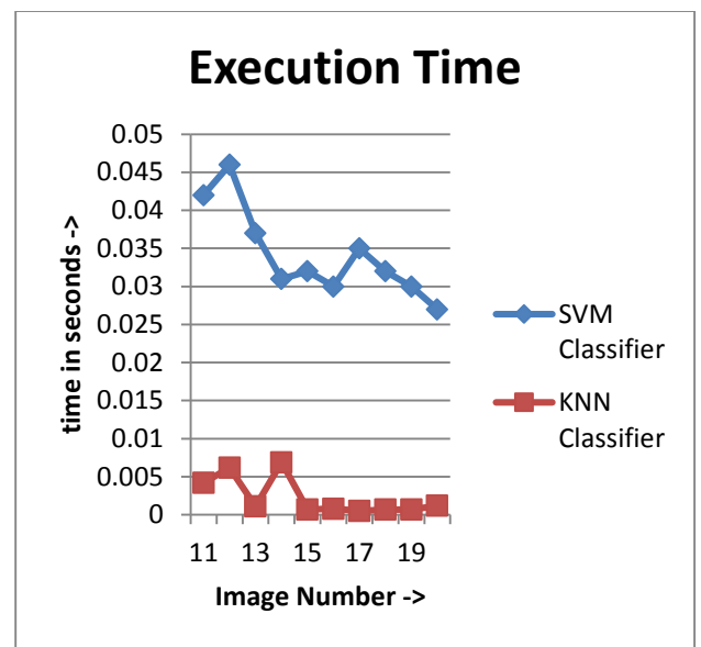
Fig.2: Execution Time
