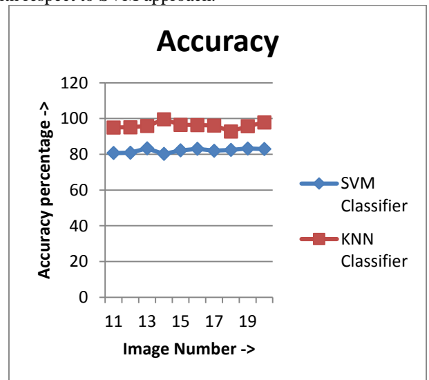
Fig.3: Accuracy Comparison
