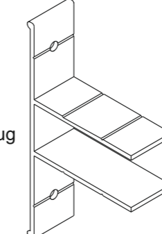
P5303 (TD3045) Midrail Fixing Lug Aluminium
