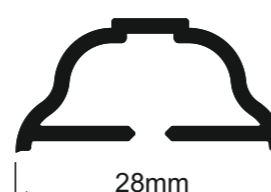
3850 28mm PVC-U snap on Georgian Bar
