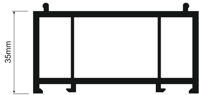
3636 35mm Frame Extender PVC-U
