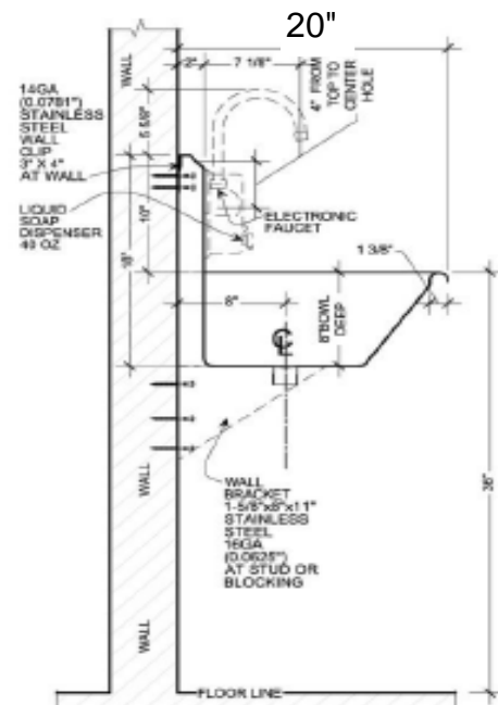
WALL MOUNT
