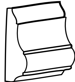
CHAIR PROFILE NO. : MS1506 PART NO. : T603 SIZE: 7/16" X 1-1/2"
